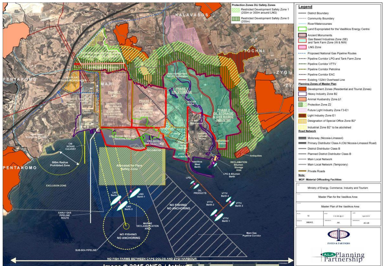
Figure: Master Plan of the Vasilikos Area.
